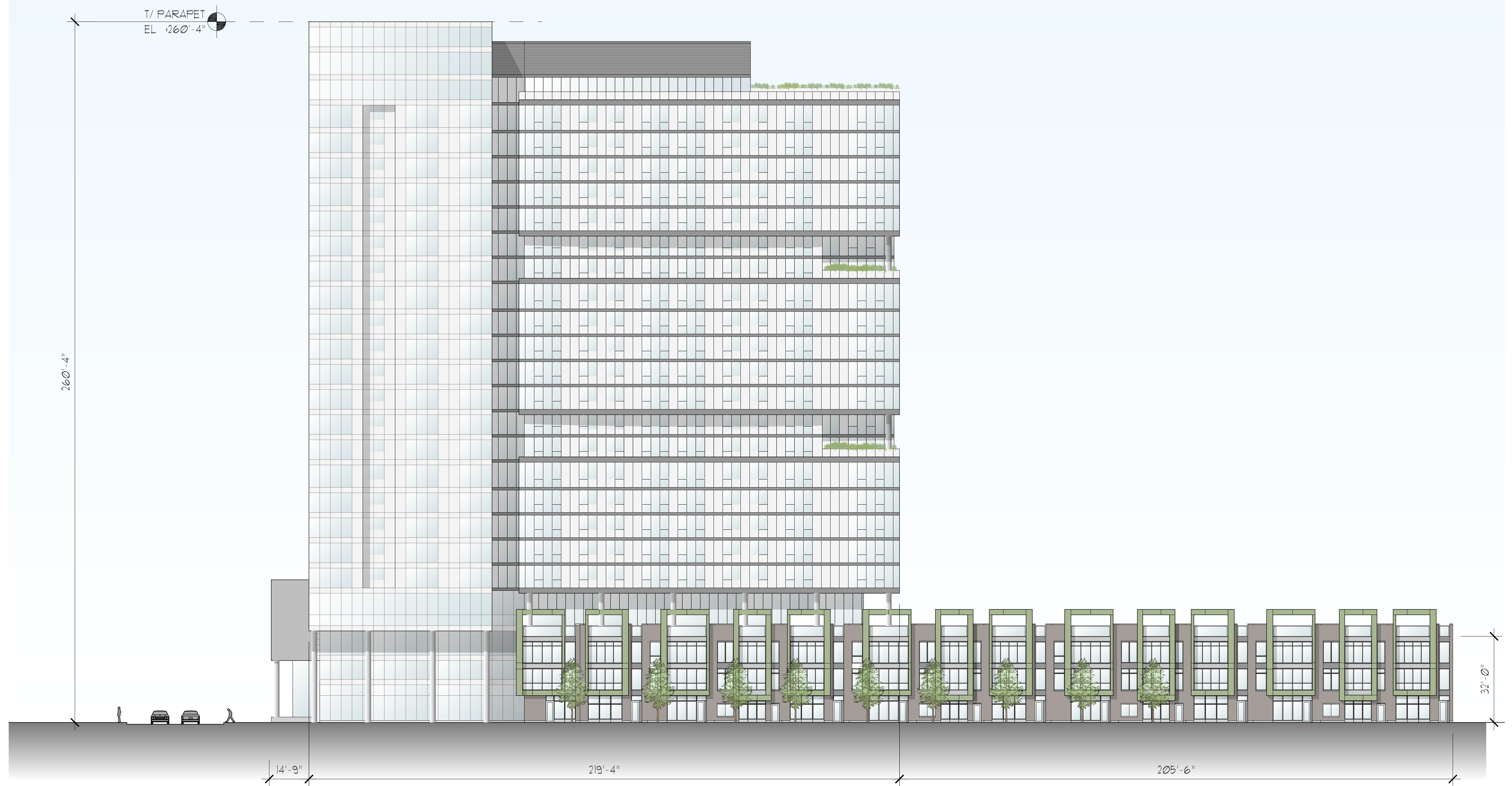
○ NORTH ELEVATION SCALE: 1" = 20'
