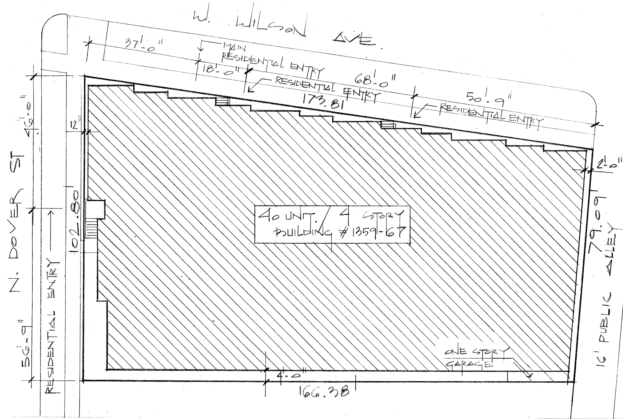
⊕ SITE PLAN 1" = 20'-0"
