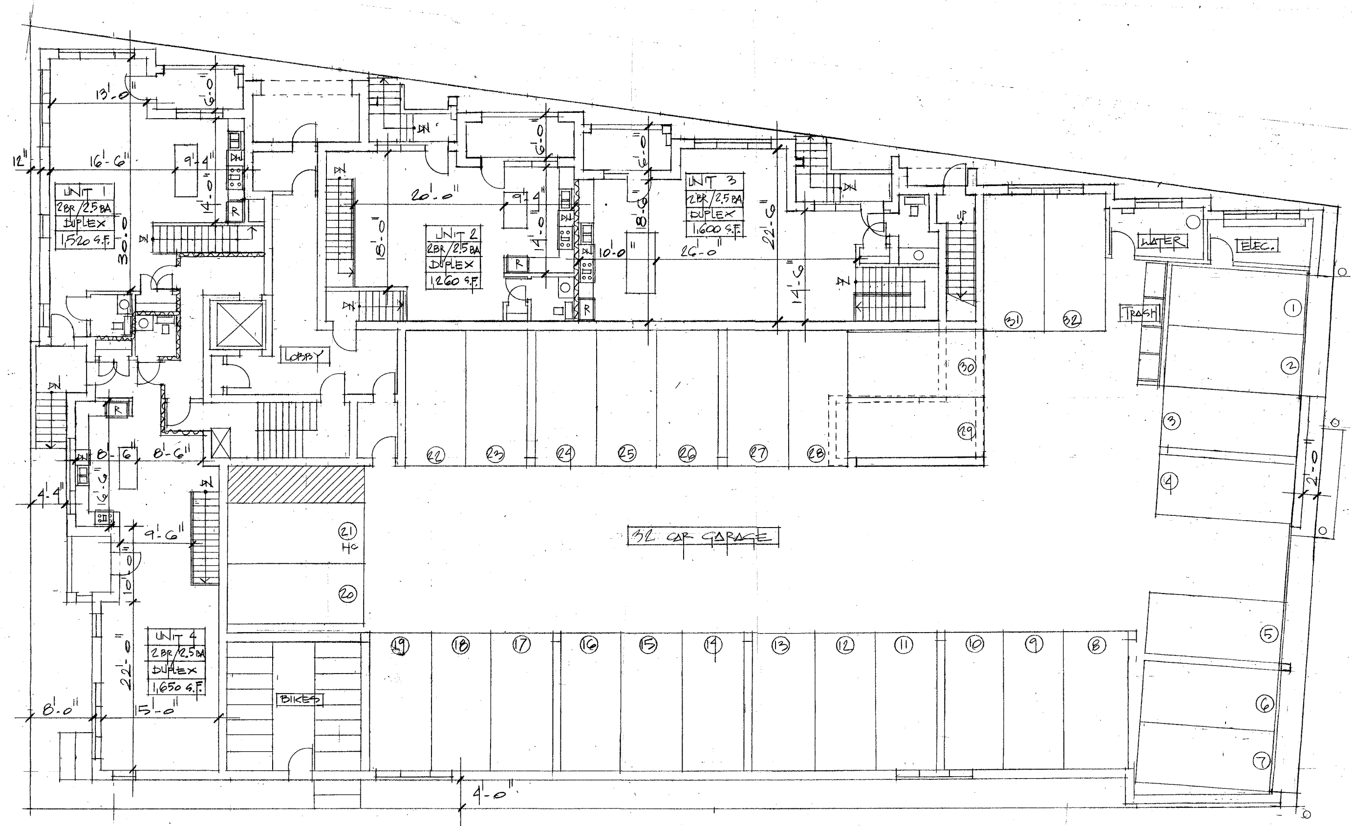
1 ST FLOOR PLAN - 5,700 S.F. 1/8" = 1'-0"
