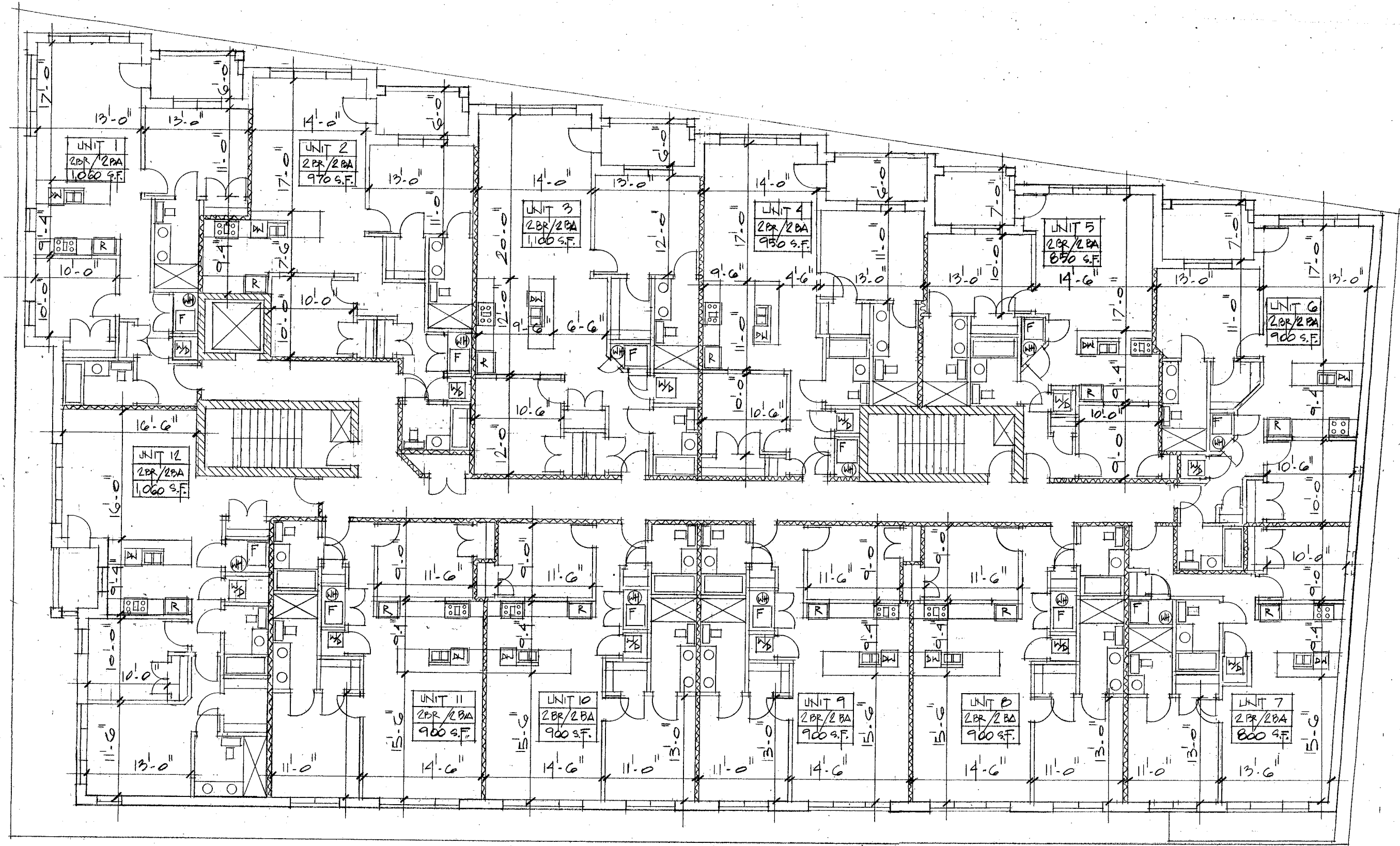
2 ND 3 RD 4 TH FLOOR PLAN - 13,500 S.F. 1/8" = 1'-0"
