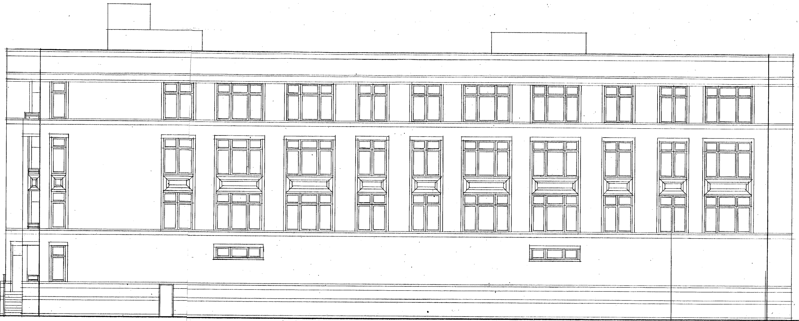
○ SOUTH ELEVATION 1/8" = 1'-0"
